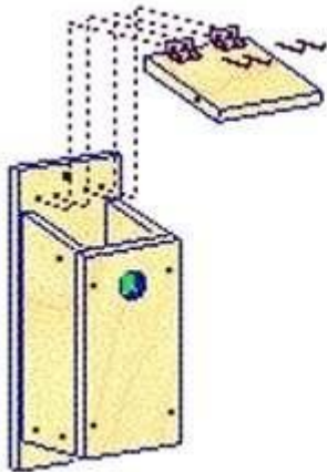
6) Fasten Roof and Hinges to Back Panel.
