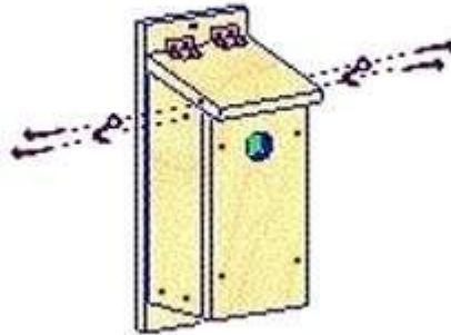
7) Fasten Shutter Hooks to Roof and Sides with Round-head Screws.
